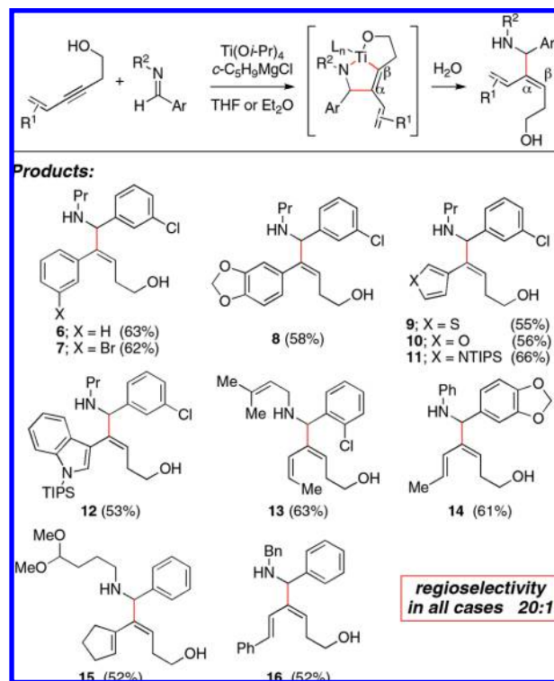
Figure 2. Alkoxy-directed union of conjugated alkynes with imines.
