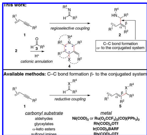
Figure 1. Regioselective union of conjugated alkynes with imines for heterocycle synthesis.
