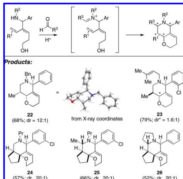
Figure 4. Cationic annulation via aza-Prins-initiated cyclization.
